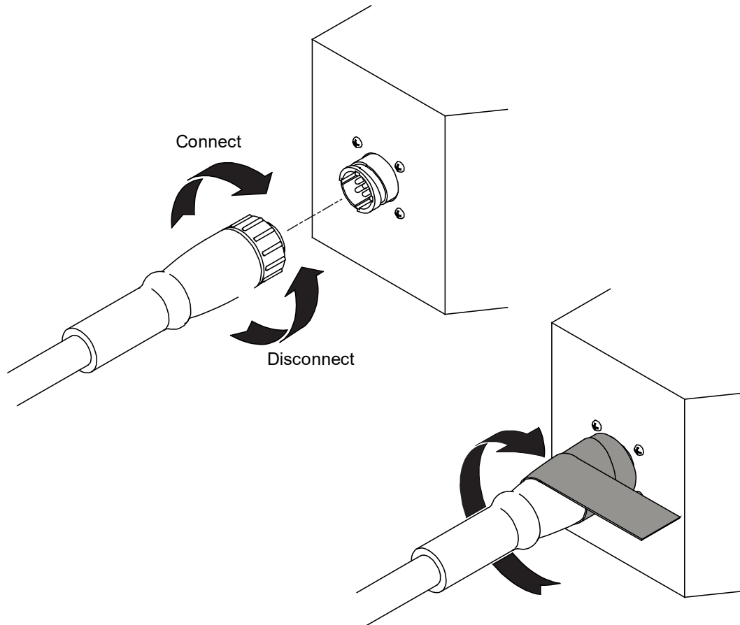
Figure 20 - Cable Connection
